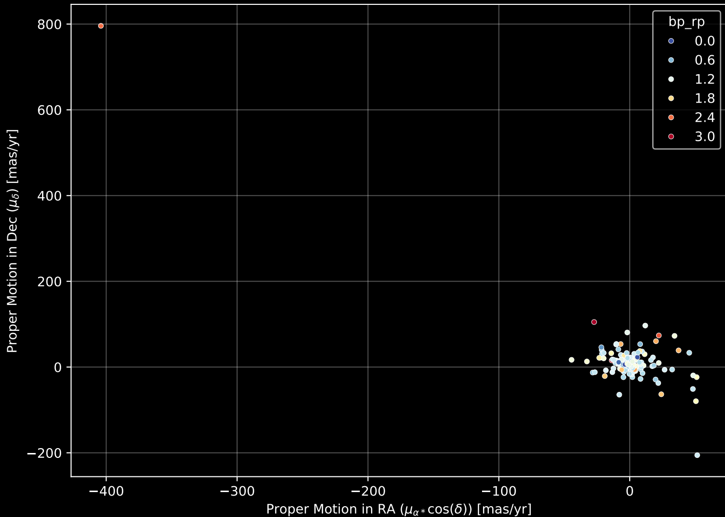
APOGEE DR17 Field: [268-24-O] Proper Motion Diagram (n= 174)
