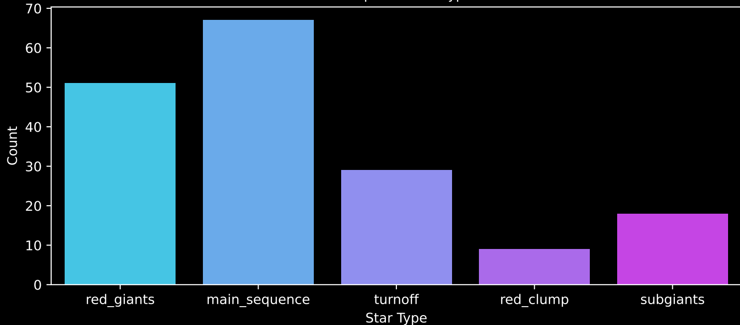
APOGEE DR17 Field: [268-24-O] Count plot of Star Type
