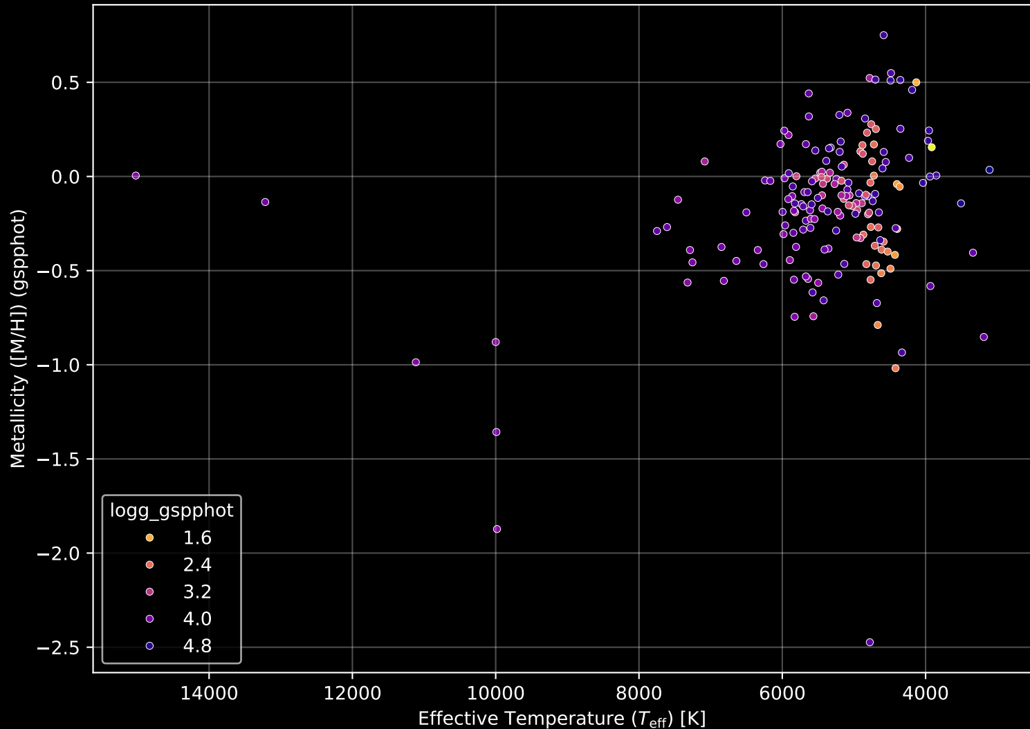
APOGEE DR17 Field: [268-24-O] Stellar Population Parameters (n= 174)
