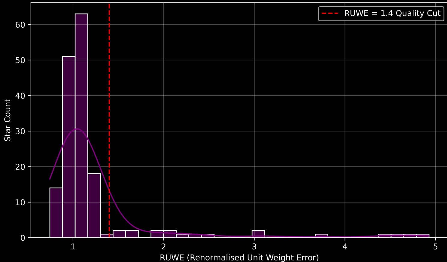
GAPOGEE DR17 Field [268-24-O] RUWE Distribution (n= 165)
