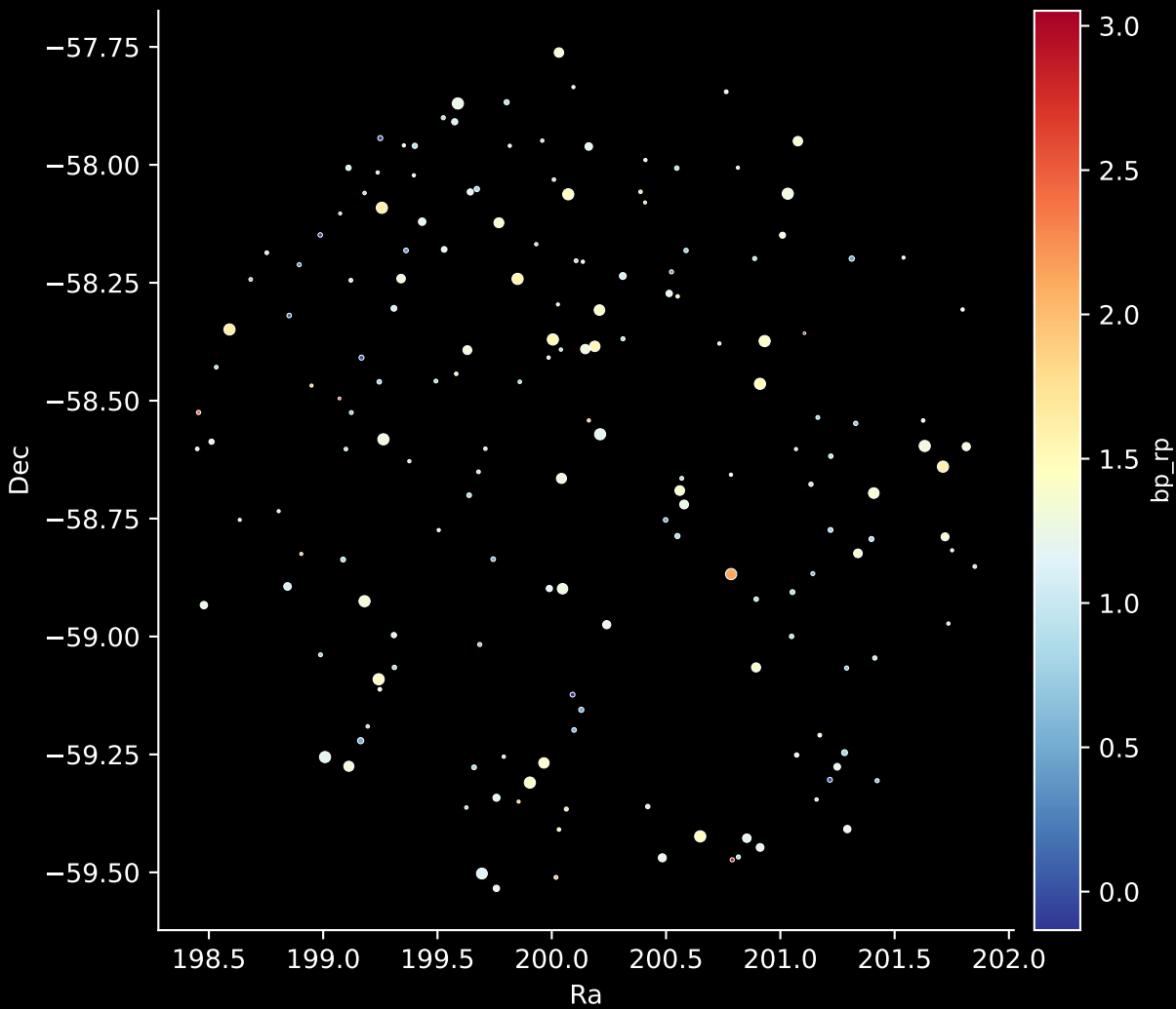
APOGEE DR17 Field: [268-24-O] Stars: 174
