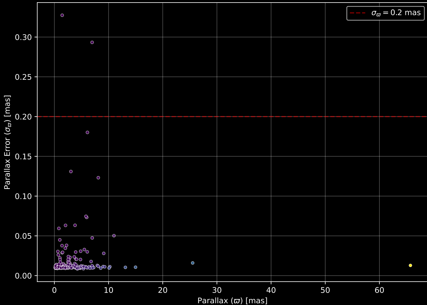
APOGEE DR17 Field: [268-24-O] Parallax Quality (n= 174)
