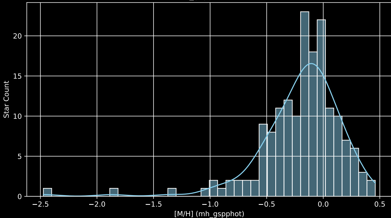
APOGEE DR17 Field: [268-24-O [M/H] (mh_gspphot) (n= 167)
